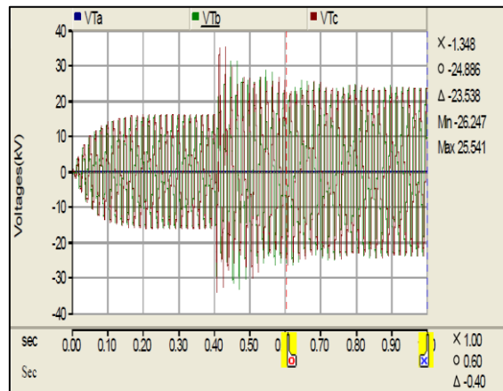
Fig 4: 6.6kV Phase Voltages of Unloaded Tertiary Winding Of 73 Mva Transformer With Lg Fault At 13.8kv Switchgear.
