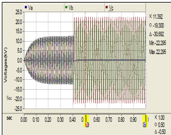
Fig 2: 13.8kv Phase Voltages at al-Adel S/S For Lg Fault at al-Adel 13.8kv Switchgear
