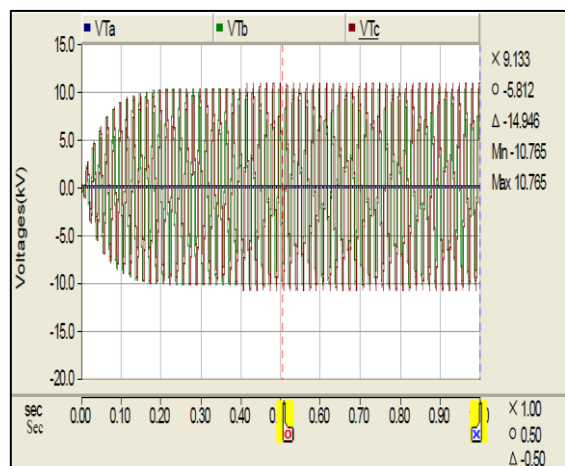
Fig 4: 6.6kV Phase Voltages of Unloaded Tertiary Winding Of 73 Mva Transformer With Lg Fault At 13.8kv Switchgear.
