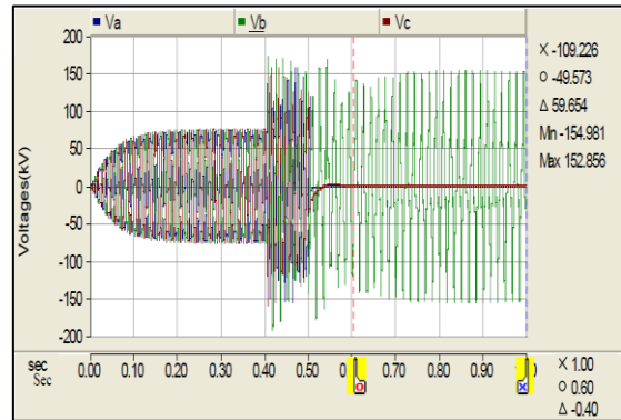
Fig 1: 110kV Phase Voltages for Load Rejection and Llg Fault at 110kv Substation
